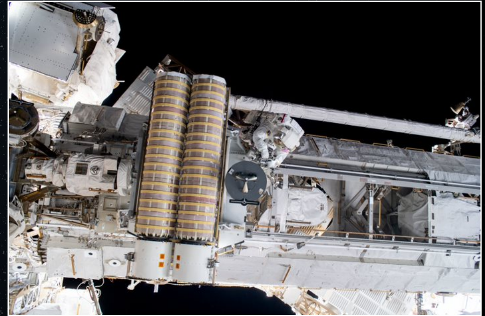
IROSA wings 5 and 6, seen here on the International Space Station, were installed in June 2023. (Credit: NASA)
