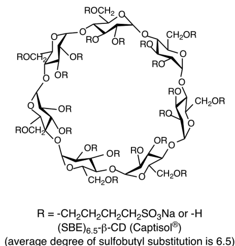
Fig. 1. Chemical structure of sulfoethyl ether-β-cyclodextrin (SBE 6.5 -β-CD), commercially known as Captisol®, with an average degree of substitution of 6.5.
