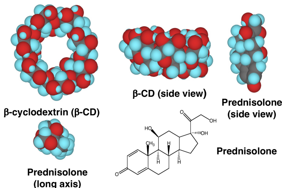
Fig. 3. Space filling model structure of \beta -cyclodextrin ( \beta -CD) and prednisolone, a steroid. Upper left: view down the short axis from the secondary face ( 2^\circ face) of \beta -CD. Upper center: a side view of \beta -CD. Top right: space-filling model of prednisolone, side view. Bottom left: space-filling model of prednisolone along the long-axis showing its fit in the torus of \beta -CD. Bottom right: the chemical structure of the steroid, prednisolone.
