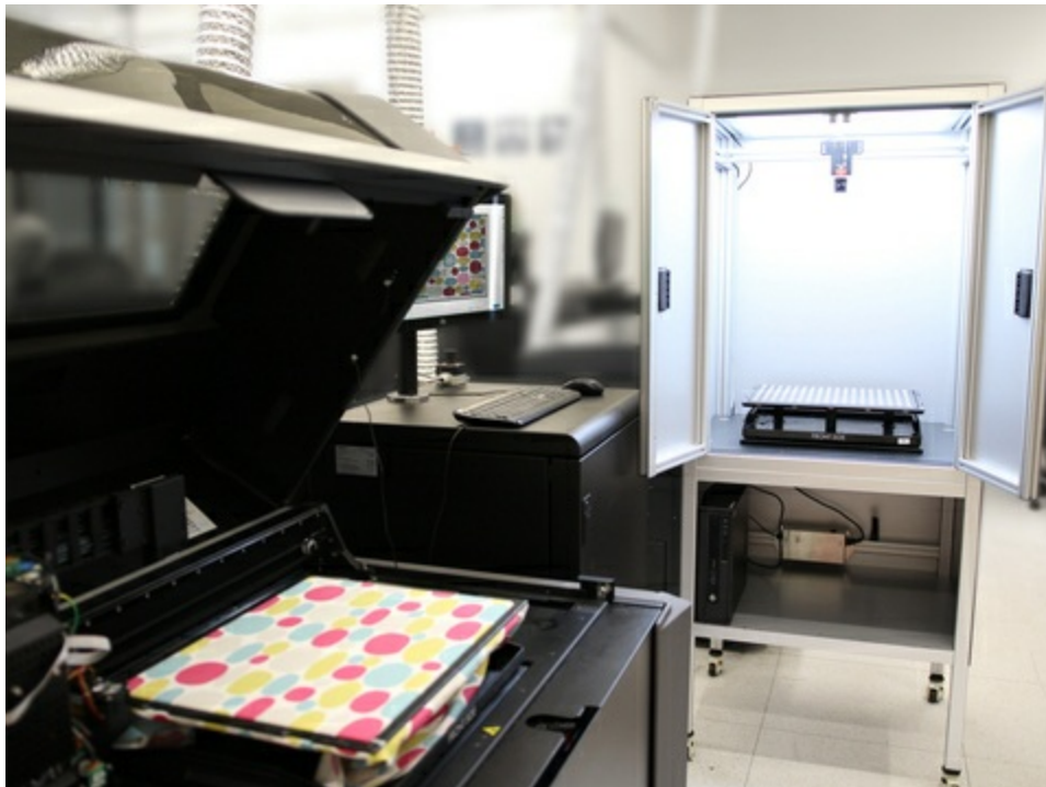
A Stratasys J850 TechStyle™ Solution with the new Fabric Alignment Station (Photo: Business Wire)
