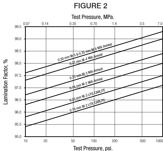
Representative lamination factors for Cleveland-Cliffs Oriented Electrical Steels at various pressures.
