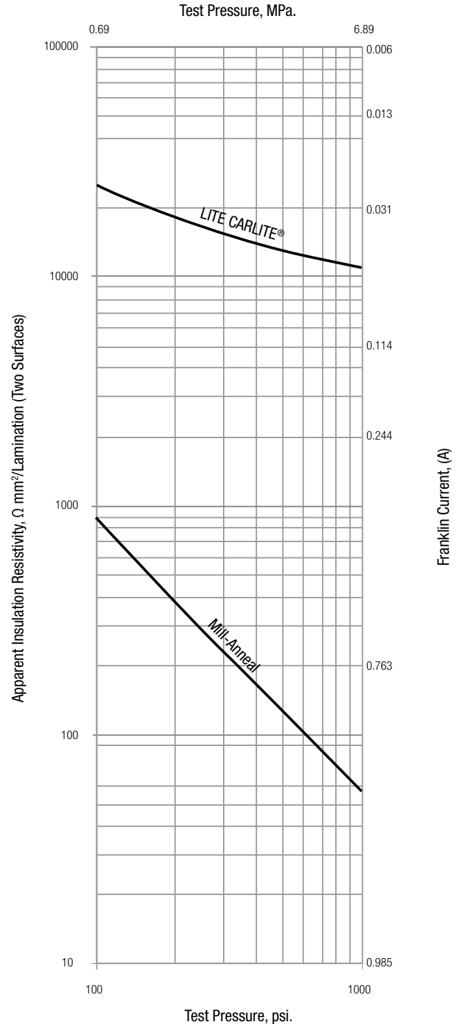
Typical surface insulation characteristics of Cleveland-Cliffs Oriented Electrical Steels at various pressures as determined by the Franklin Test.
