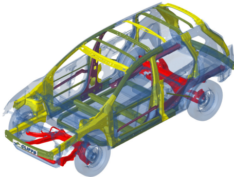
Car model design based on 2020 Nissan Rogue FE Model developed by Center for Collision Safety and Analysis at George Mason University.
