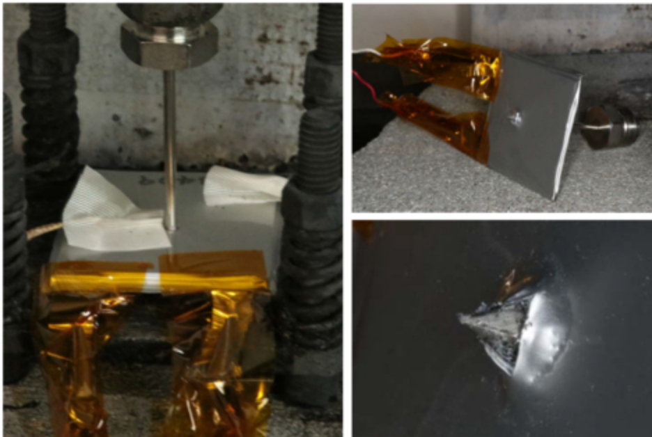
Amprius Technologies Passes Military Performance Specification Nail Penetration Test with Unprecedented 390 Wh/kg Cell (Photo: Business Wire)
