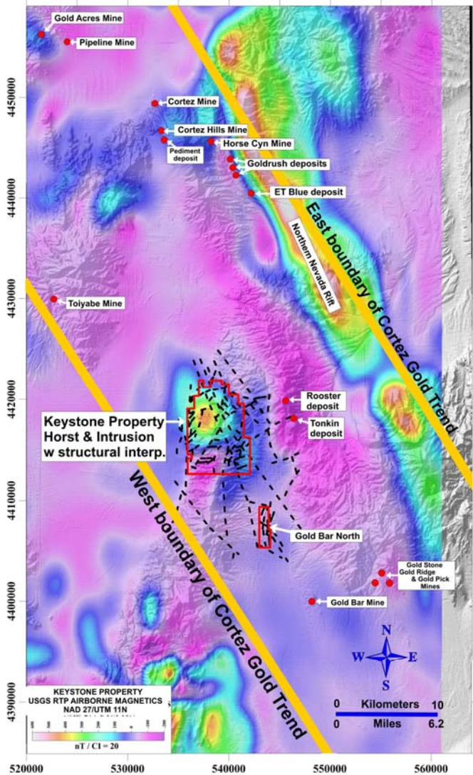
Regional Aeromagnetics
