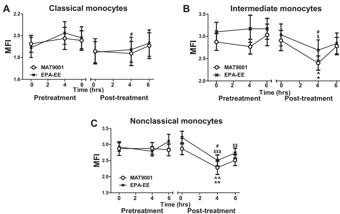
Figure 6 Effects of MAT9001 or EPA-EE treatment on monocyte CCR5. CCR5 MFI levels were examined on monocytes (subsets: classical [A], intermediate [B], and nonclassical [C]) by flow cytometry in the fasting (0 hour) and postprandial (4 and 6 hours after the high-fat meal) states. * P < .05 , ** P < .01 for posttreatment vs pretreatment of MAT9001; # P < .05 for posttreatment vs pretreatment of EPA-EE; P < .05 , ^{*}P < .01 for 4 or 6 hours vs 0 hour of MAT9001 treatment; ^{*}P < .05 , ^{**}P < .01 , ^{***}P < .001 for 4 or 6 hours vs 0 hour of EPA-EE treatment.
