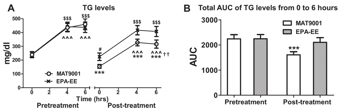
Figure 1 Effects of MAT9001 or EPA-EE treatment on postprandial TG levels. (A) Blood triglyceride (TG) levels were measured fasting (0 hour) and postprandially (4 and 6 hours after the high-fat meal) just before (pretreatment) and at the end of (post-treatment) each treatment. (B) For each intervention, total area under the curve (AUC) of TG levels from 0 to 6 hours was compared between pre- and post-treatment values. *** P < .001 for posttreatment vs pretreatment with MAT9001; # P < .05 for posttreatment vs pretreatment with EPA-EE; $$$ P < .001 for 4 or 6 hours vs 0 hour of MAT9001 treatment; $$$ P < .001 for 4 or 6 hours vs 0 hour of EPA-EE treatment. †† P < .01 for MAT9001 vs EPA-EE for posttreatment vs pretreatment.
