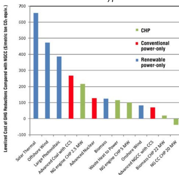
Figure 5: Comparing Costs of Reducing GHG Emissions Across Resource Generation Type
