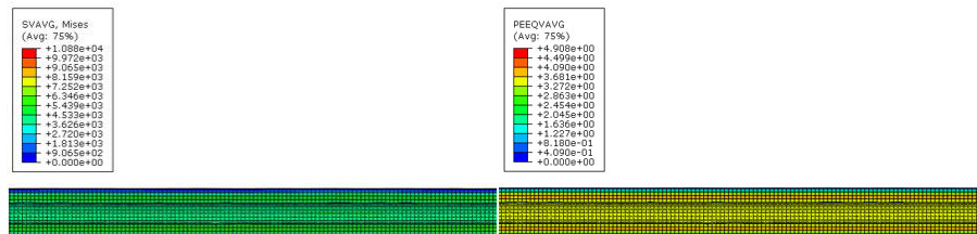
Figure 7. Long Billet with Clad High Reduction Extrusion Clad Steady-State Front Section: Stress (psi, left) and Plastic Strain (right).
