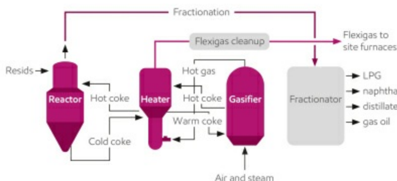
The FLEXICOKING process (Graphic: Business Wire)
