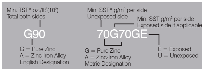
FIGURE 1 – COATING DESIGNATION
