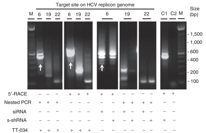
Figure 3 Evidence of on-target mode of action for TT-034 by 5' RACE. Electrophoretic analysis of 5' RACE products and nested PCR re-amplification of 5' RACE products generated on the HCV replicon RNA genome on account of the action of TT-034, transfected synthetic siRNA analogues or transfected synthetic shRNA analogues (s-shRNA) of shRNA6 (target 6), shRNA19 (target 19), and shRNA22 (target 22). The control lanes correspond to 5' RACE amplification using primers specific for target site 6 in the presence of synthetic shRNA19 (lane C1), or in the absence of TT-034 using primers for the target site of shRNA19 (lane C2). White arrows identify 5' RACE products generated by shRNA6 versus full-length HCV replicon RNA (large molecular weight bands).
