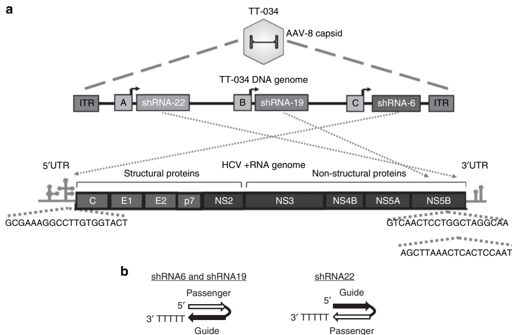
Figure 1 Genome organization and target site location of TT-034, a recombinant AAV8 vector encoding three shRNA targeting the HCV genome. (a) The viral genome of AAV8 has been replaced by 3 expression cassettes separated by Pol III termination sequences and stuffer regions. The contents of the expression cassettes are from 5' to 3': modified U6-9 Pol III promoter (box A) driving shRNA22 expression targeted to the HCV NS5B region (viral RNA-dependent RNA polymerase), modified U6-1 Pol III promoter (box B) driving shRNA19 expression, also targeted to the NS5B region and modified U6-8 Pol III promoter (box C) driving shRNA6 targeted to the 5' UTR of HCV. The expression cassettes are flanked by inverted tandem repeats derived from AAV4 at the 5' end and AAV2 at the 3' end of the genome. (b) Schematic representation of the expressed hairpin polarity. The guide strand is defined as the strand targeting the (+) RNA HCV genome.
