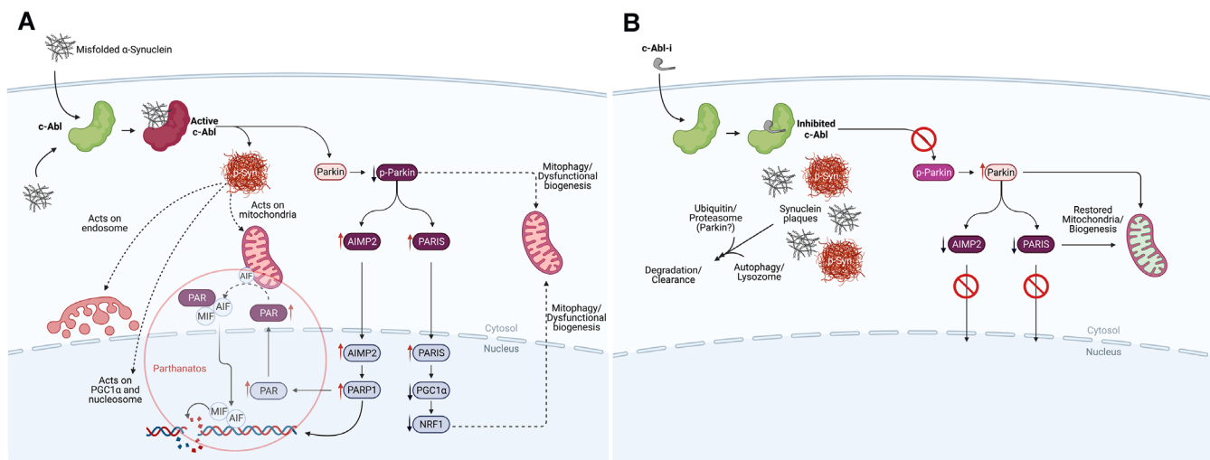
FIG. 3. The biochemistry of Parkinson's disease initiation and progression and how to disrupt it. (A) The process of neurodegeneration. Misfolded \alpha -synuclein can arise from a variety of factors (see text). Misfolded \alpha -synuclein may form within the neuron or by transfer through cell surface receptors or by crossing membrane bilayers. Within a neuron, misfolded \alpha -synuclein is 'sensed' and c-Abl activated, driving the formation of pathologic \alpha -synuclein by chemical modification (p-Syn). 28 Chemical modification creates a form of \alpha -synuclein that represents the pathologic species of the disease leading to disruption of mitochondrial integrity, negatively impact the endosome, disrupt nucleosomal structure and modulate transcription of certain genes. 32-38,63-72 C-Abl also inactivates parkin by chemical modification, which affects mitochondrial quality control and suppresses protein clearance mechanisms. 28-34,77-79 Parkin inactivation suppresses the complex interplay between parkin and pink1 at the mitochondrion, which act in concert to maintain mitochondrial integrity, quality and regulate mitochondrial biogenesis. 77 Parkin inactivation leads to the accumulation of toxic parkin substrates, such as the parkin interacting substrate (PARIS), the aminoacyl tRNA synthetase complex-interacting multifunctional protein 2 (AIMP2) and the far upstream element-binding protein 1 (FBP1). 28-34,77-79 PARIS and AIMP2 accumulate in adult conditional parkin knockout mice and MPTP-intoxicated mice as well as in patients with PD. Increased levels of PARIS can lead to mitochondrial dysfunction through downregulation of the peroxisome proliferator-activated receptor- \gamma coactivator (PGC)-1 \alpha transcriptional co-activator protein and loss of DA neurons in a PARIS-dependent manner. PGC1- \alpha is a transcriptional co-activator that plays a central role in regulation of energy metabolism. Overexpression of AIMP2 leads to an age dependent, selective degeneration of DA neurons through activation of poly (ADP-ribose) polymerase 1 (PARP1), driving PARP1-mediated parthanatos. This suggests that PARIS and AIMP2 may be important contributors to the loss of DA neurons and possibly other vulnerable neurons following parkin inactivation. Inactivation of parkin also disrupts protein clearance mechanisms through autophagy, lysosomal, and proteasomal degradation pathways. (B) The consequences of c-Abl inhibitor treatment on the process of neurodegenerative disease. Inhibition of c-Abl precludes c-Abl activation, blocking the build-up of toxic parkin substrates PARIS and AIMP2 and terminating downstream events. This also re-establishes normal mitochondrial quality control and biogenesis. Model studies demonstrate that modified and unmodified \alpha -synuclein aggregates are shunted to lysosomal or proteasomal degradation pathways for clearance with concomitant recovery of motor function.
