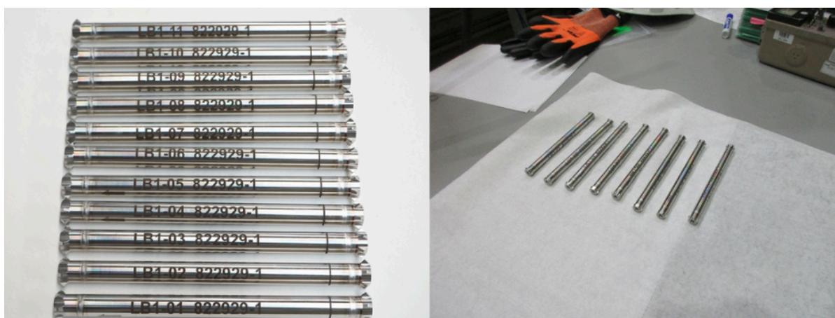
Capsules containing Lightbridge Fuel material samples before loading into an experimental assembly.
