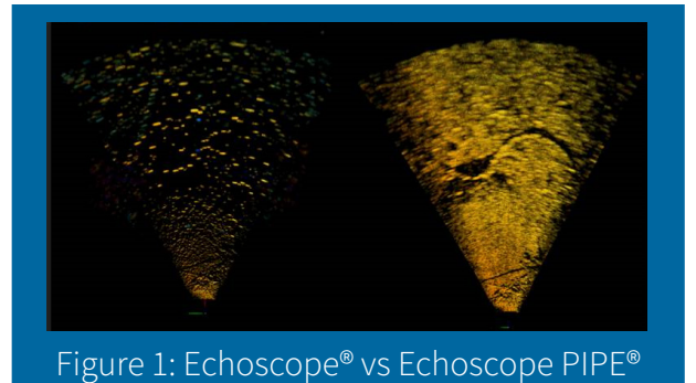
Figure 1 which is a single ping from our Echoscope® shows the increased density of data from PIPE compared to our previous generation of sonars.
