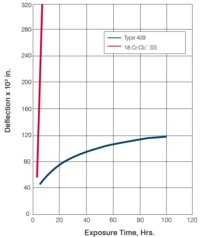
FIGURE 1 – 1600 °F (671 °C) SAG TEST
