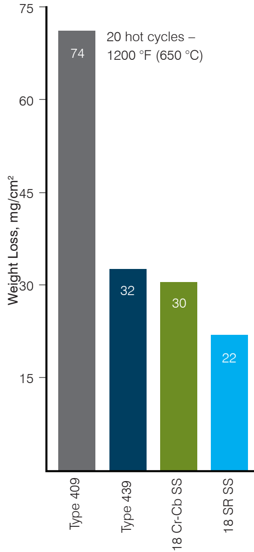
FIGURE 4 –HOT SALT CORROSION TEST
