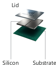
2D package
