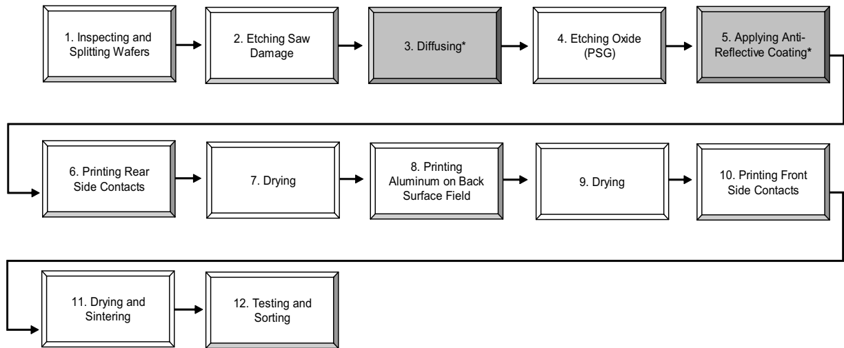
Solar Cell Manufacturing Process Flow Chart
